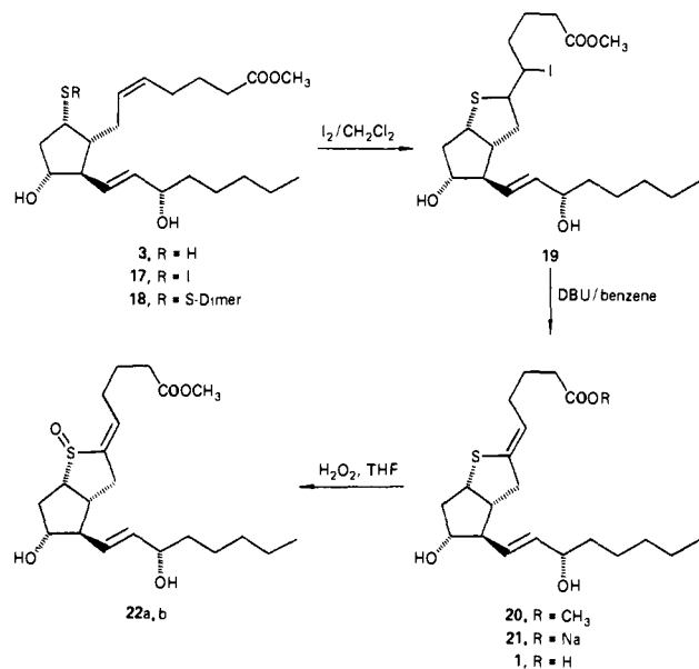
Figure 5. Synthesis of (5 Z )-6,9-thiaprostacyclin.
