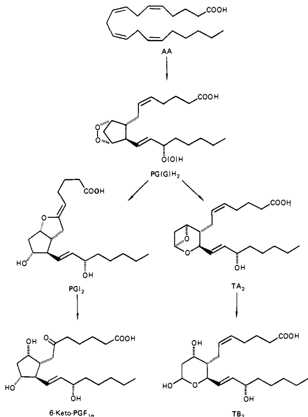
Figure 1. Biosynthesis of prostacyclin (PGI 2 ) and thromboxane A 2 (TA 2 ).
